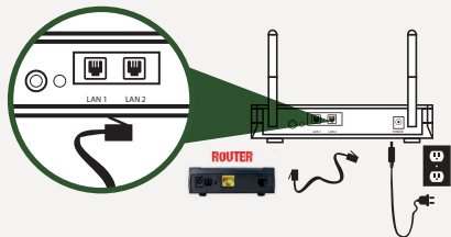
1.2 - Connect the network cable from the WAP to your router using either LAN1 or LAN2.
